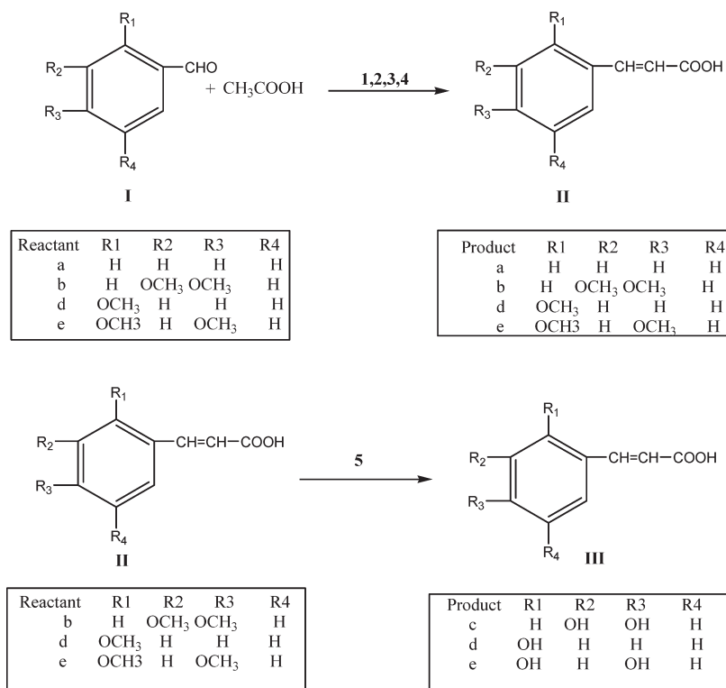
Scheme 1. Synthesis of Cinnamic Acids from Acetic Acid and Substituted Benzaldehydes (IIa–b, IIIc–e) a
